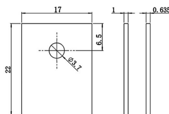
TO-247
