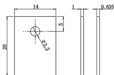
TO-220
