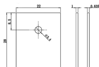
TO-264
